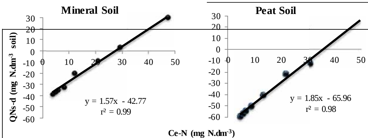
Figure 2: Ammonium-N sorption isotherms: Amount of ammonium- N sorbed or desorbed (QNs-d) against soil equilibrium concentration of ammonium ions (Ce-N)
