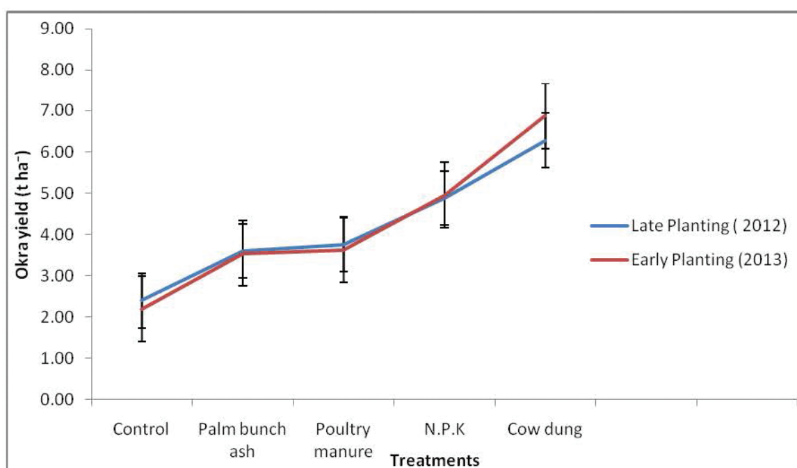
Fig. 2: Effect of treatments on the cumulative yield of okra ( \text{t ha}^{-1} )
