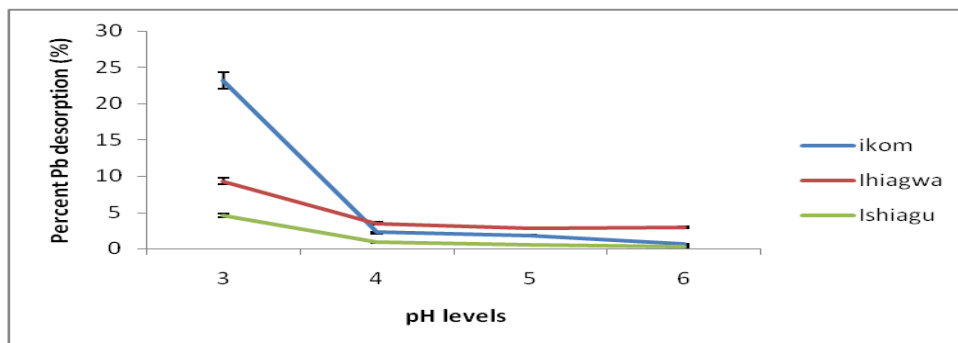
Fig 3: Percent desorption of lead at different pH levels
