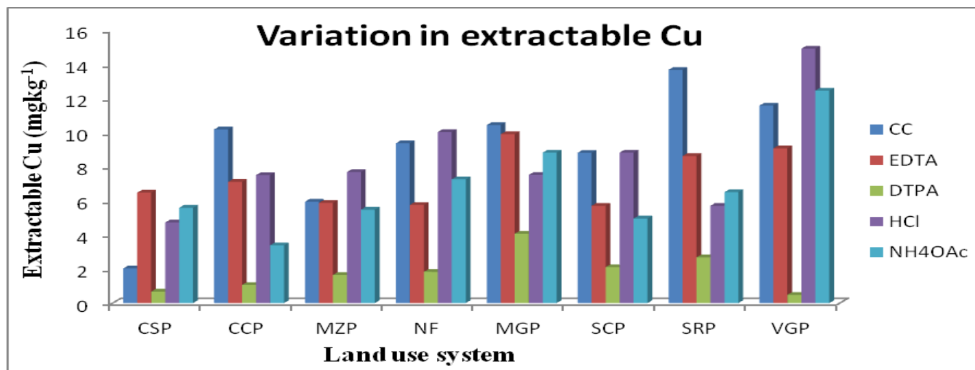
Figure 1: Effect of land use on the variability of extractable Cu under long-term farming systems
