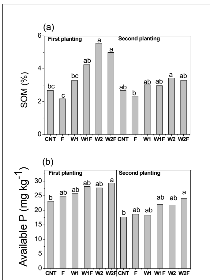
Fig. 1: Soil organic matter (SOM) (a) and available P (b) at the end of the first and second growth of maize ( Zea mays L.). Means across treatments with similar letter(s) are not significantly different ( p < 0.05 ) from each other. CNT: control; F: fertilizer; W: water hyacinth compost; 1: 2.5 t ha -1 ; 2: 5.0 t ha -1 .
