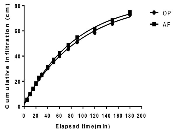
Fig. 2: Average cumulative infiltration for soil under oil palm and arable farm
