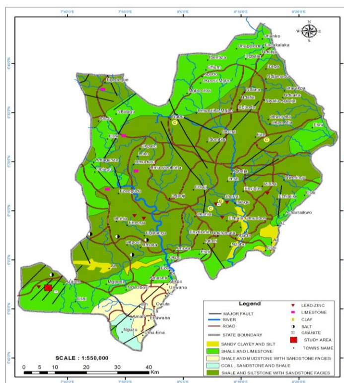
Figure 2. Geological and mineral resources map of Ebonyi State showing lead–zinc occurrences and the location of the study area. Source: Geological Survey Agency of Nigeria (2006).
