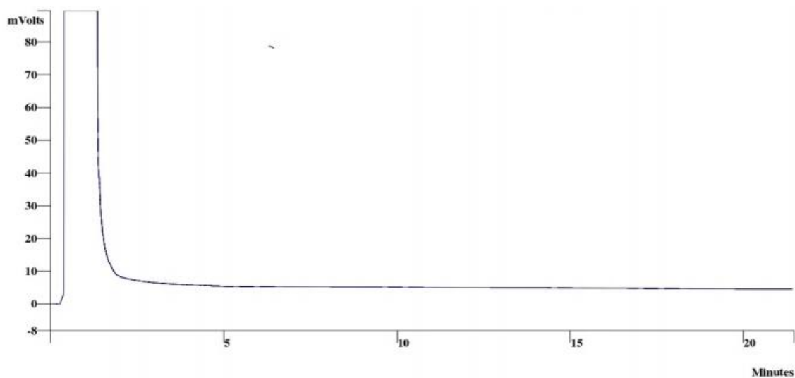
Fig. 5: Chromatogram of the TPH for BD3
