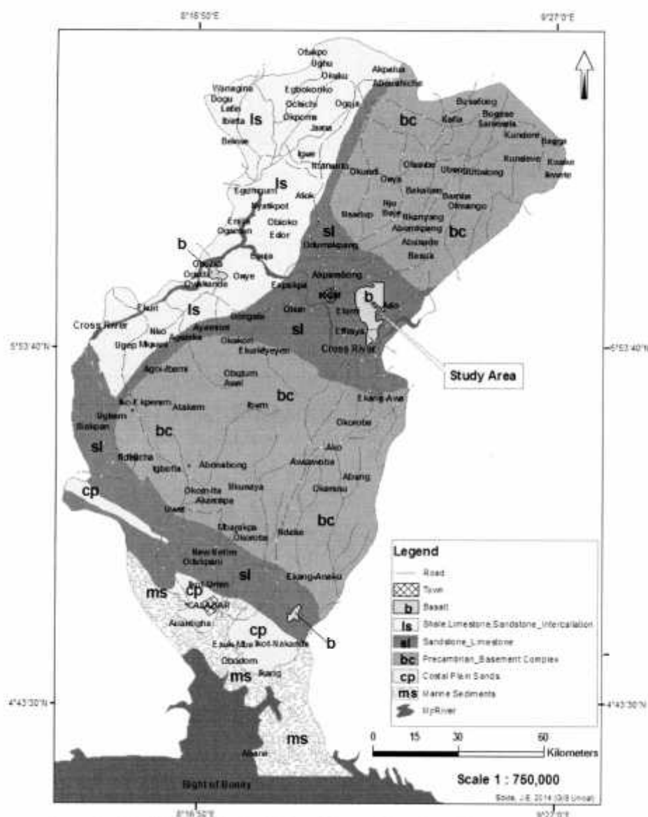
Figure 1: Simplified Geological Map of Cross River State Showing Location of Study Area at Ikom
