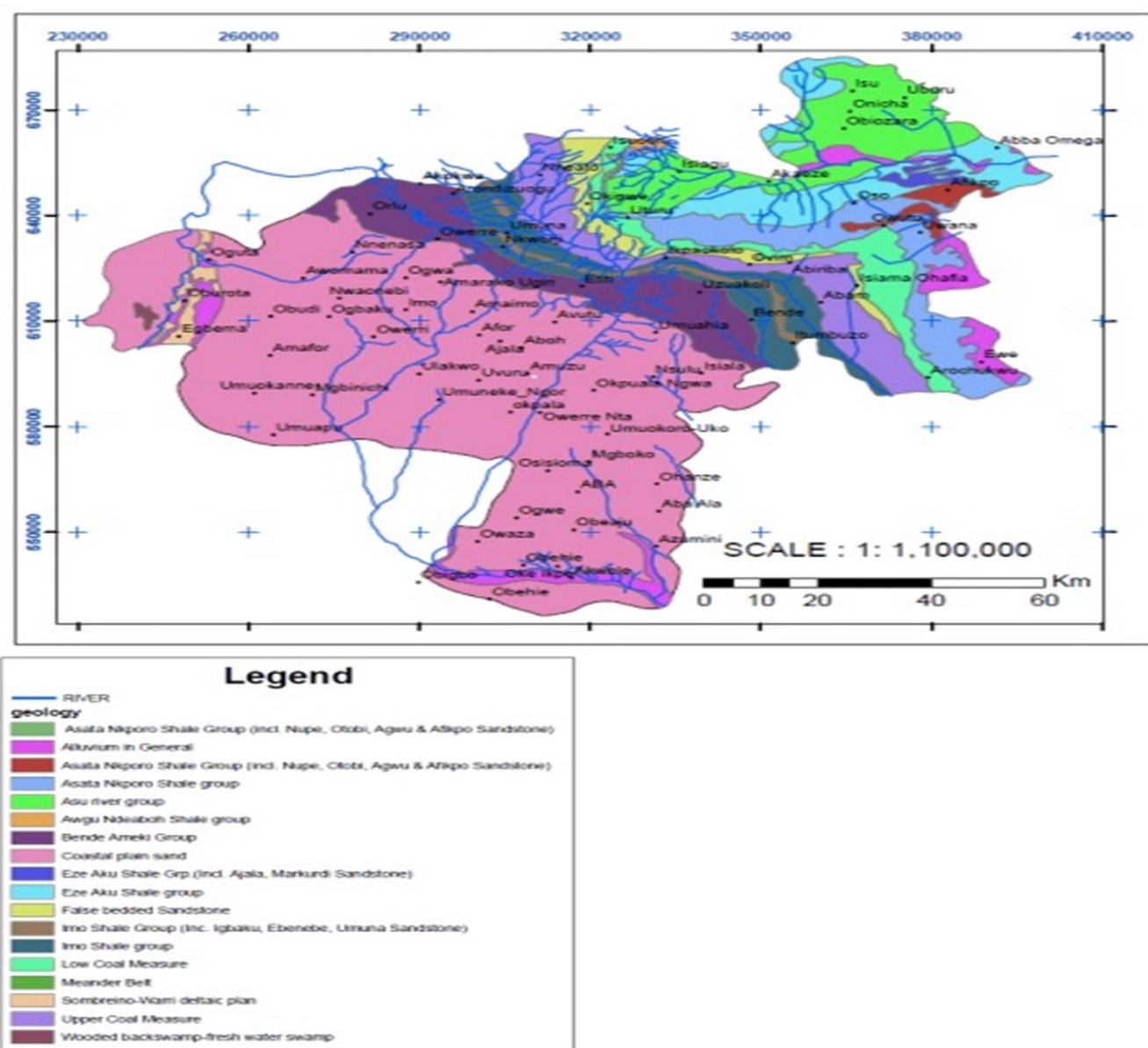
Fig 1: Geological map of old Imo State showing the study area, Ahukaemere et al. , 2015
