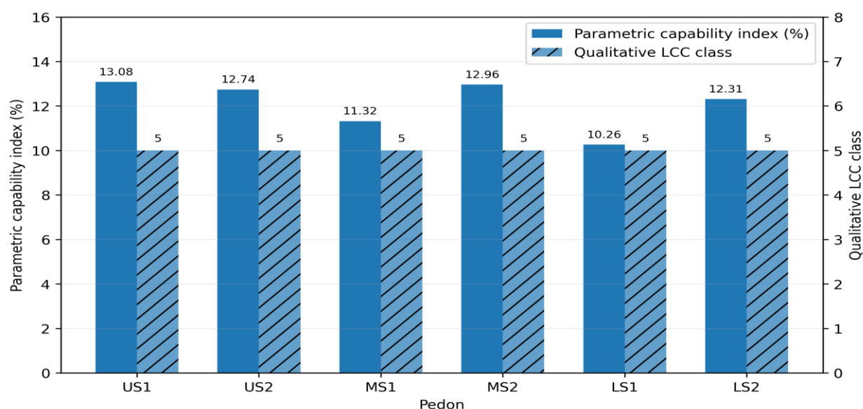
Figure 2. Comparison of parametric capability indices and qualitative capability classes. The left axis reports the parametric capability index (%) and the right axis reports the qualitative capability class (I–VIII). The pedons are Class V under the qualitative assessment and Class VII under the parametric index.
