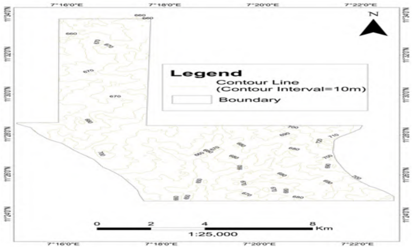
Figure 7: Contour map of the study area
