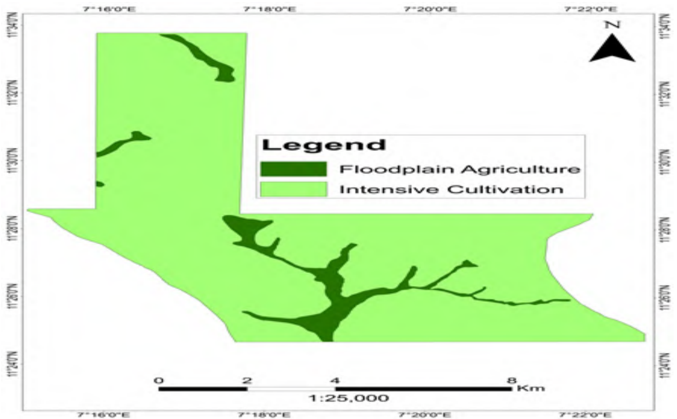
Figure 8: Land use map of the study area
