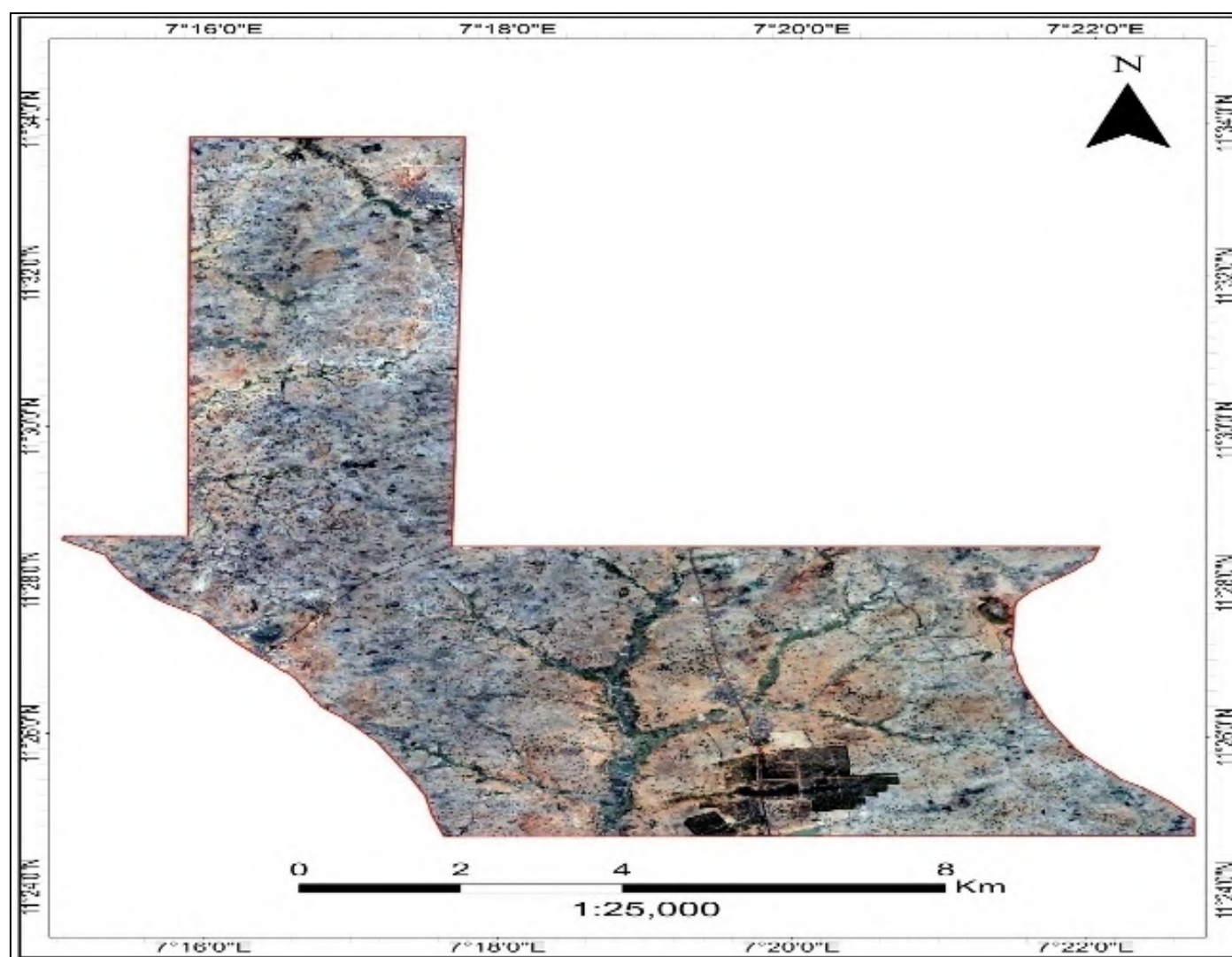
Figure 5: Landsat imagery of the study area
