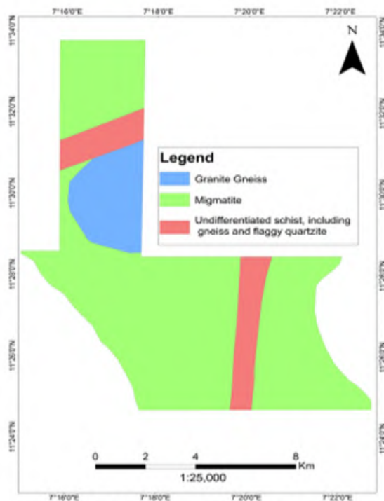
Fig. 2: Geological map of study area
