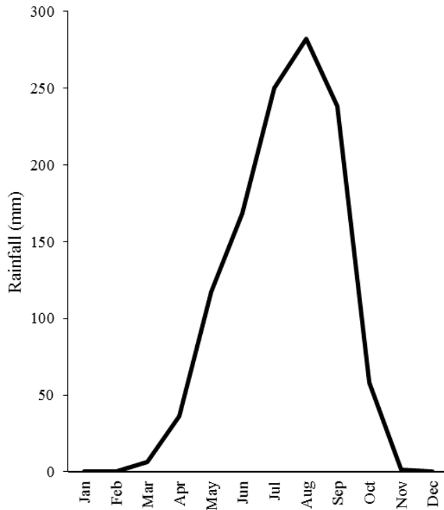
Figure 3: Long-term (1964-2013) rainfall data of the study area
