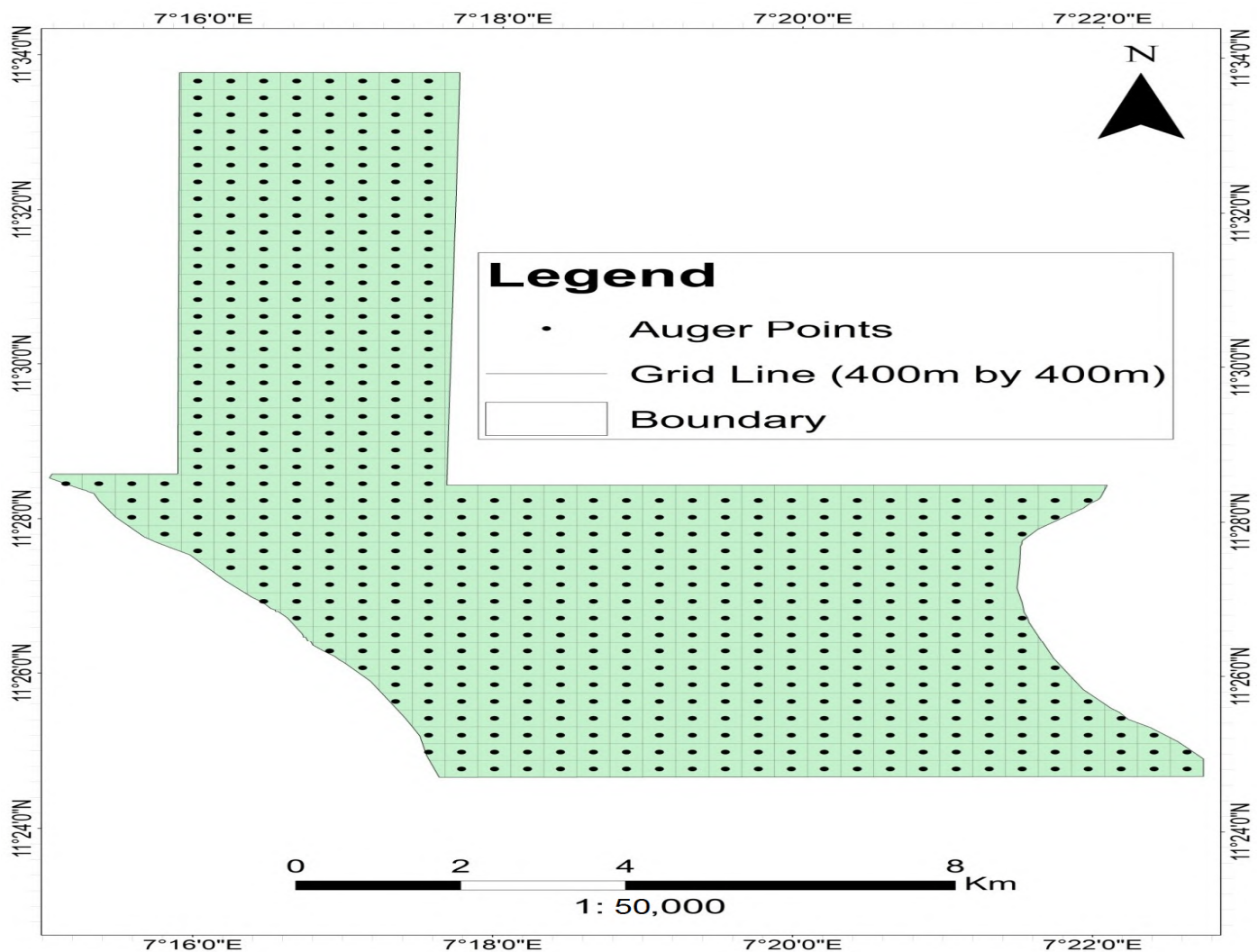
Figure 9 Base map of the study area
