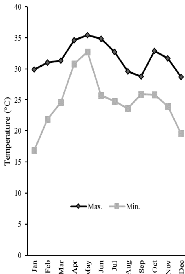
Figure 3: Long-term (1964-2013) temperature data of the study area
