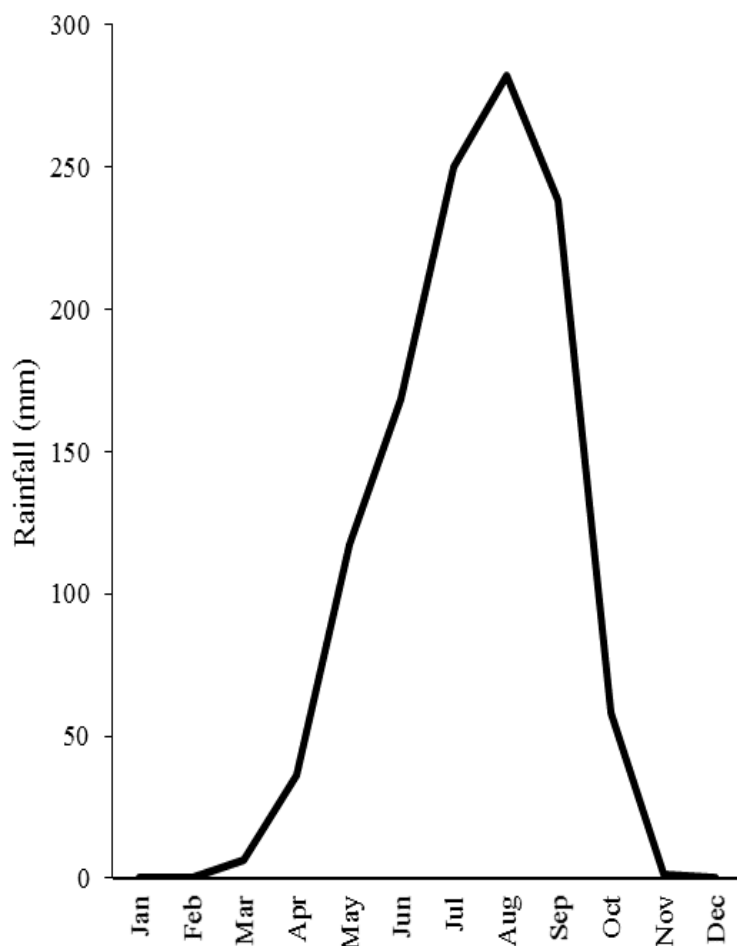
Figure 2: Long-term (1964-2013) rainfall data of the study area
