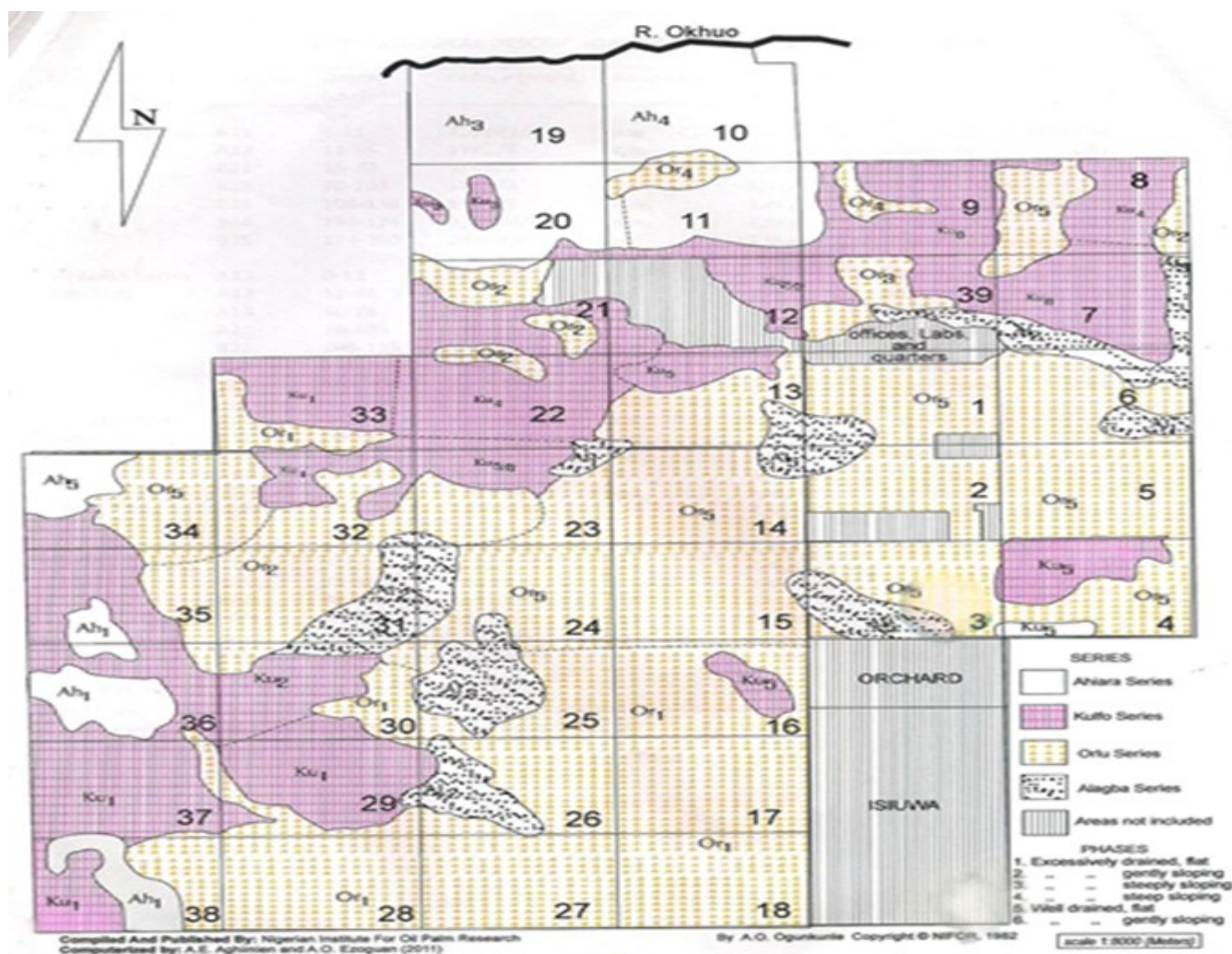
Fig. 1: Soil Map of NIFOR Main station
