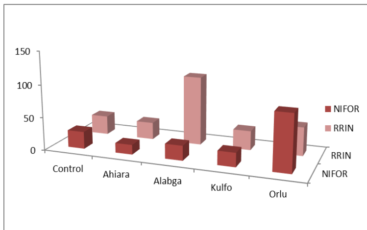
Figure 3. Soil Organic Carbon Stocks (SOCS) affected by Soil types in g/ kg
