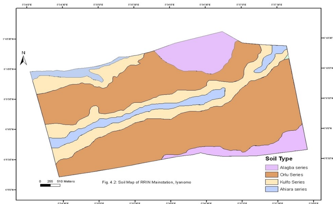
Fig. 2: Soil Map of RRIN
