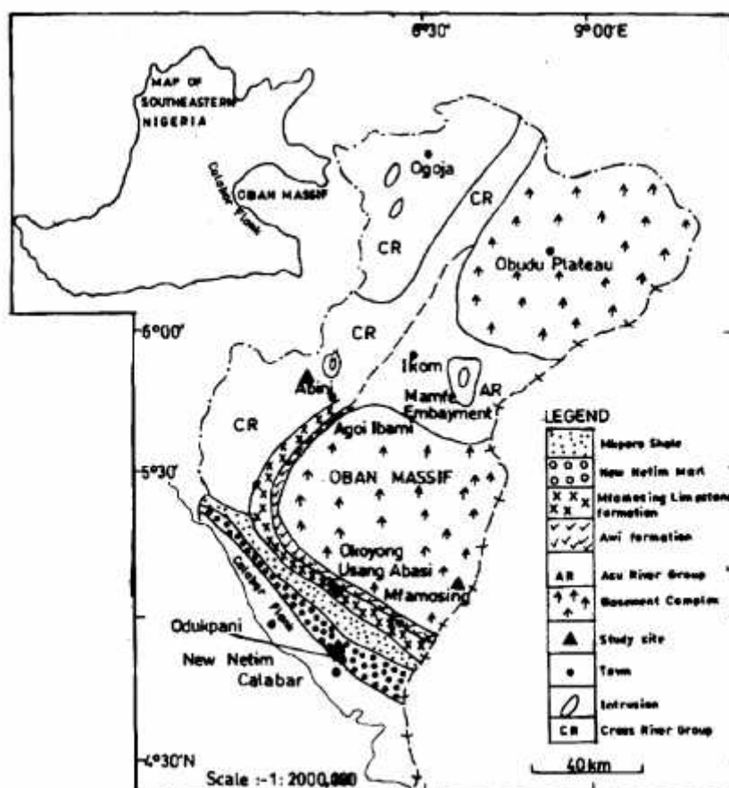
FIG.1: Geological map of Cross River State showing the study areas
