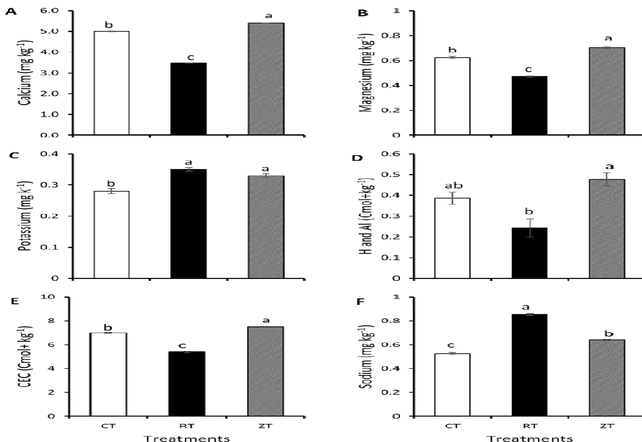
Figure 3: Means ( \pm standard error) of A (Calcium), B (Magnesium), C (Potassium), D (Hydrogen and Aluminium), E (CEC) and F (Sodium) as influenced by tillage practices. Means with different letters on the same char differed significantly from one another according to the LSD at 5% level of significance.
