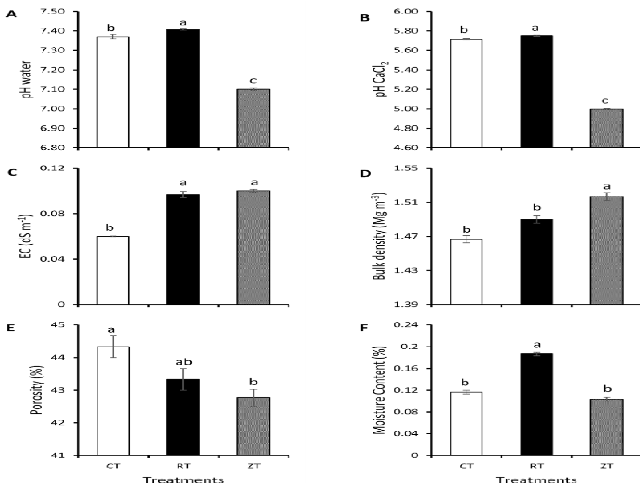
Figure 1: Means ( \pm standard error) of A (pH water), B (pH \text{CaCl}_2 ), C (Electrical conductivity), D (Bulk density), E (Porosity) and F (Moisture Content) as influenced by tillage practices. Means with different letters on the same char differed significantly from one another according to the LSD at 5% level of significance.
